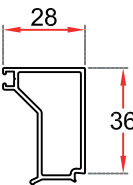
90.3570 JUNQUILLO MARCO
