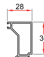
90.3570 JUNQUILLO MARCO
