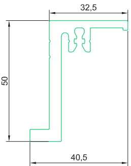
20.1100 MARC
