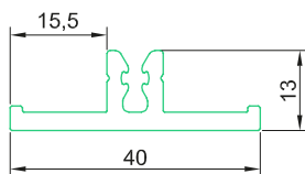
20.3900 TRANSVERSAL EXTERIOR
