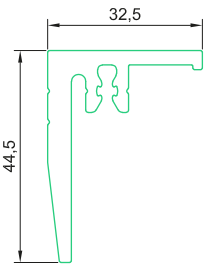
20.2100 FULLA
