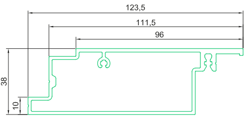
20.2200 ACOBLAMENT PORTA
