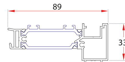
89.3580 INVERSOR HOJA
