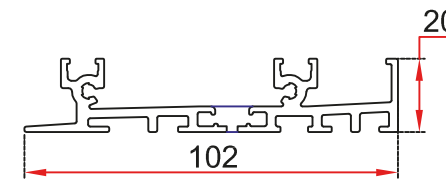
78.8300 MARCO SOLERA
