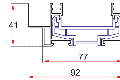
78.1212 MARCO GALANDAGE
